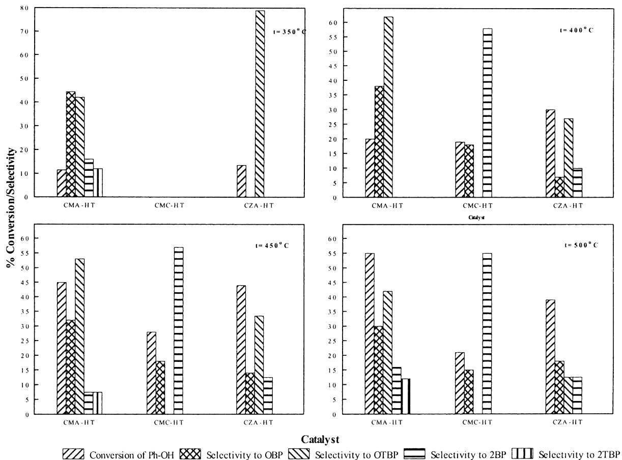
Fig. 4. Effect of temperature on the t -butylation of phenol over the calcined hydrotalcites: OBP, O -butenyl phenol; OTBP, O-tert -butyl phenol; 2BP, 2-butenyl phenol; 2TBP, 2- tert -butyl phenol.
