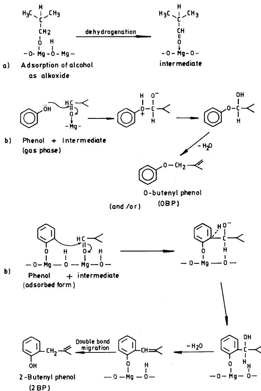
Fig. 5. A plausible mechanism for the formation of butenyl phenols.
