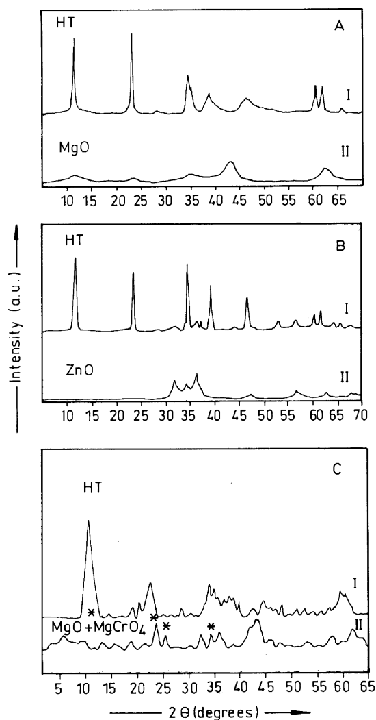
Fig. 1. The X-ray powder diffractograms of: (A) MA-HT (I) and CMA-HT (II); (B) ZA-HT (I) and CZA-HT (II); (C) MC-HT (I) and CMC-HT (II); (*) indicates \text{MgCrO}_4 phase.
