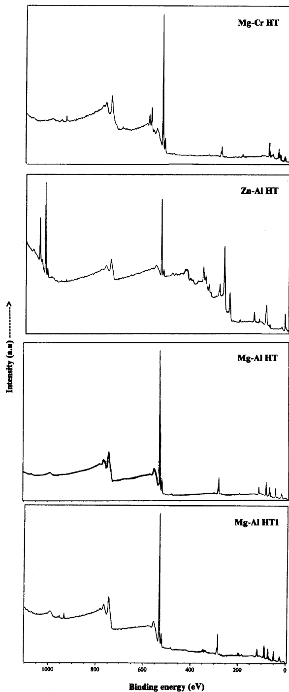
Fig. 2. The XPS spectra of MA-HT, MA-HT-1, MC-HT and ZA-HT.
