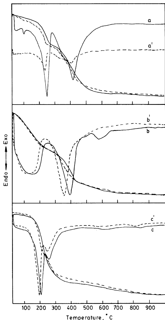
Fig. 3. The DTA/TG patterns of: (a) MA-HT (air) and (a') MA-HT (N 2 ); (b) MC-HT (air) and (b') MC-HT (N 2 ); (c) ZA-HT (air) and (c') ZA-HT (N 2 ).
